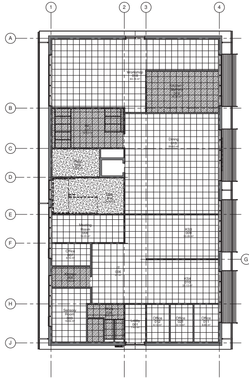
Ground Floor Plan - Ceiling Finishes Scale 1:100
