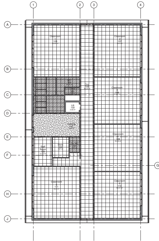
First Floor Plan - Ceiling Finishes Scale 1:100
